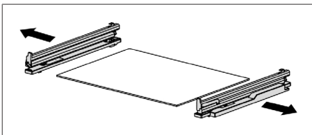
Fig. 8.3 Removing the runners from the glass
