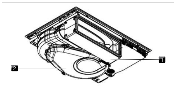
Fig. 4.2 Rear view
