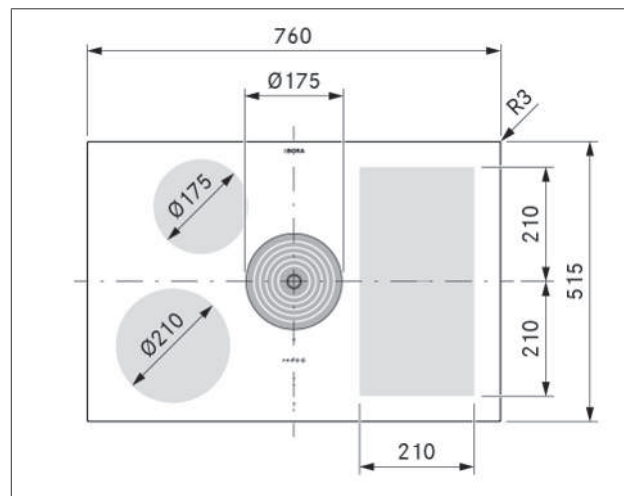
Fig. 3.1 Appliance dimensions top view
