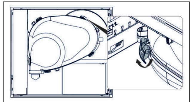
Fig. 9.21 Innsugingsrom-fester
