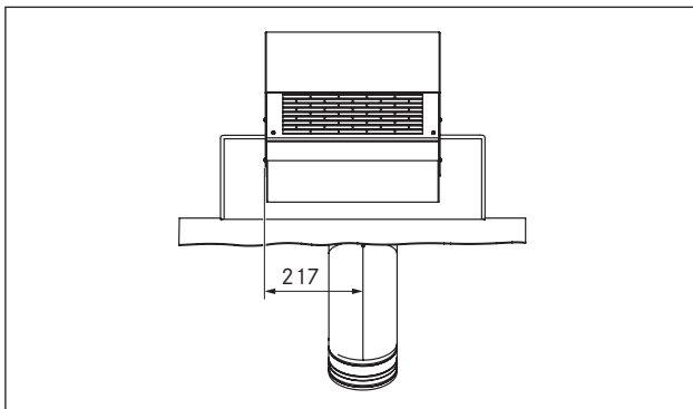
Fig. 5.1 Front view
