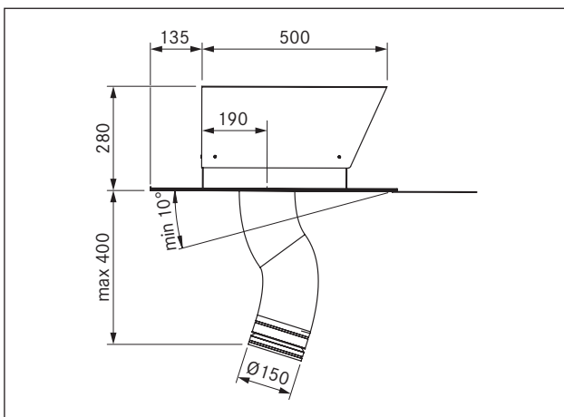
Fig. 5.2 Side view
