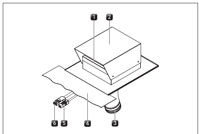
Fig. 5.1 Structure of tiled roof fan
