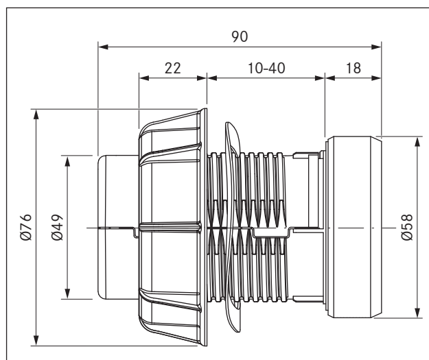
Fig. 3.8 Control knob dimensions
