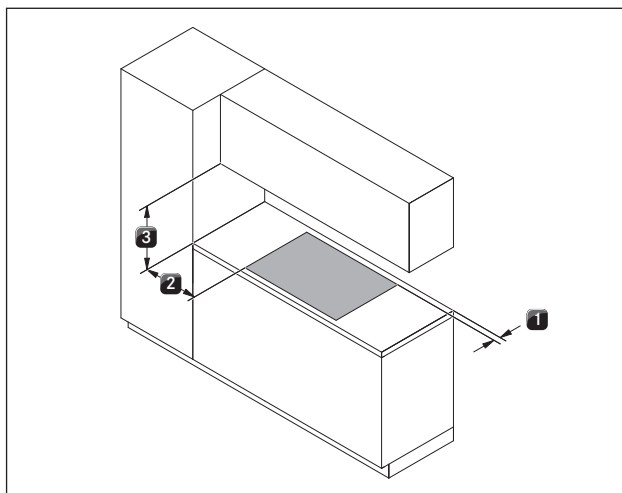
Fig. 5.1 Minimum distance
