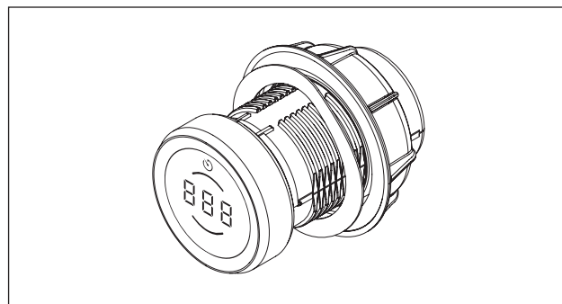
Fig. 3.7 Control knob
