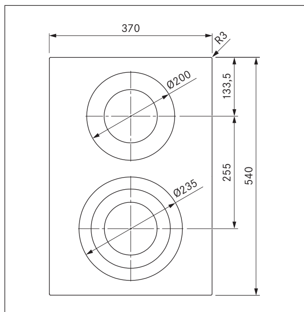
Fig. 3.1 PKC3 appliance dimensions from above
