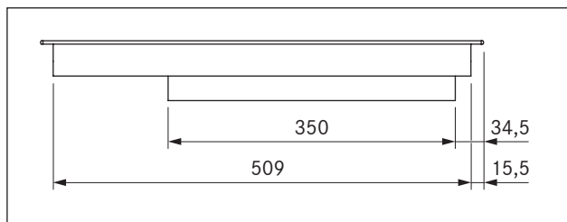
Fig. 3.6 PKCB3 appliance dimensions side view
