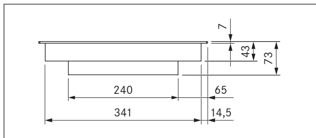
Fig. 3.5 PKCB3 appliance dimensions front view
