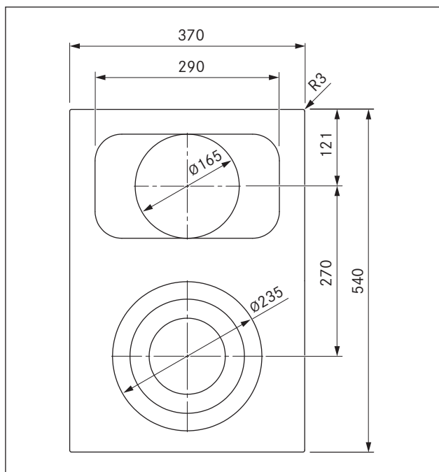
Fig. 3.4 PKCB3 appliance dimensions from above
