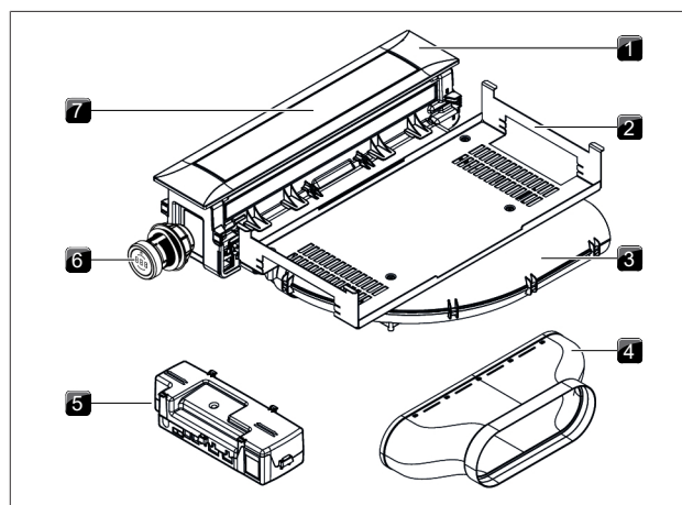
Fig. 3.5 Cooktop extractor PKA3/PKA3AB
