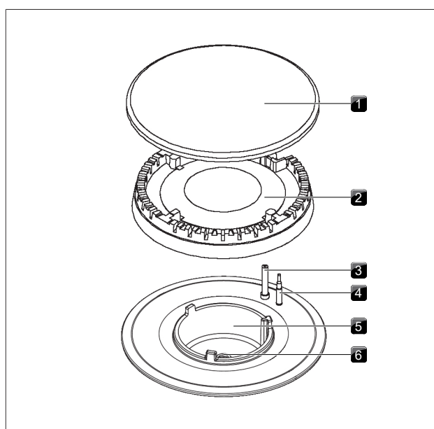
Fig. 7.7 Gas burner structure
