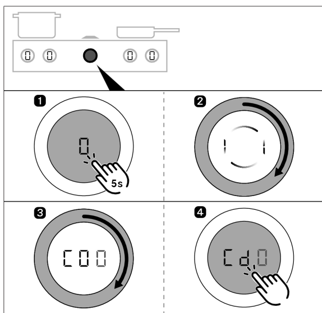
Fig. 6.8 Checking the software version
