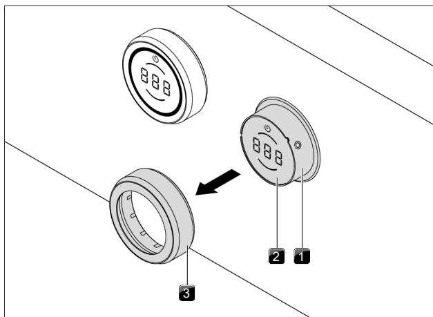
Fig. 7.8 Pull out the knob ring
