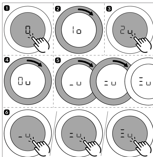
Fig. 5.32 Activating the heat retention function on radiant bodies
