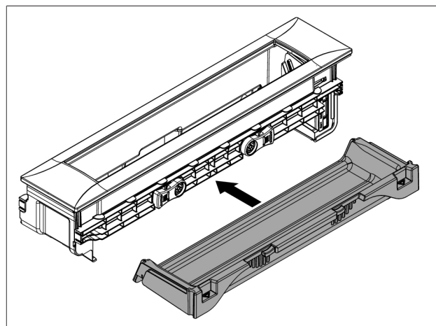
Fig. 7.5 Installing the maintenance tray
