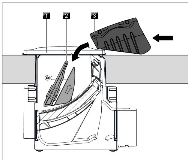
Fig. 7.3 Fitting the cover flap
