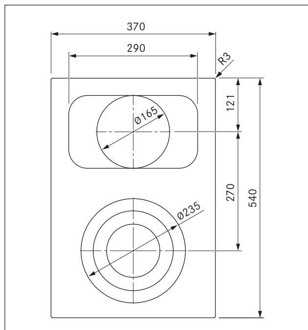
Fig. 3.4 PKC3B Device dimensions aerial view
