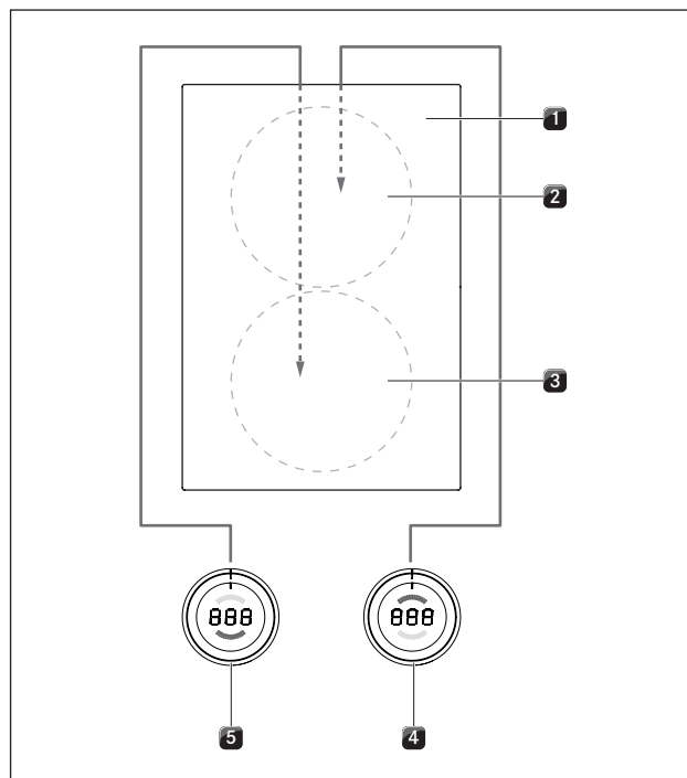
Fig. 5.21 Cooking zone connection in 180° installation
