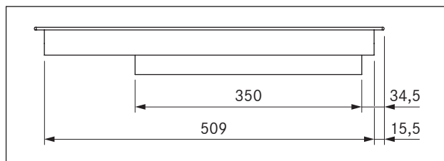
Fig. 3.6 PKC3B Device dimensions side view
