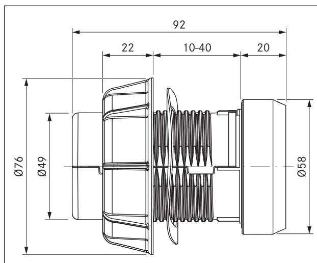
Fig. 3.7 Device dimensions control knob
