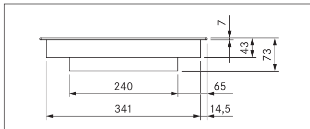
Fig. 3.5 PKC3B Device dimensions front view
