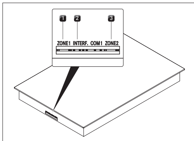
Fig. 5.19 Connections on the cooktop
