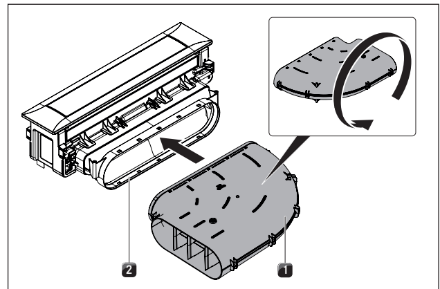
Fig. 6.27 Turn angled ducting piece
