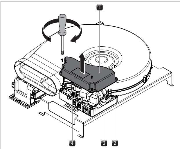
Fig. 6.37 Open the cover of the control unit
