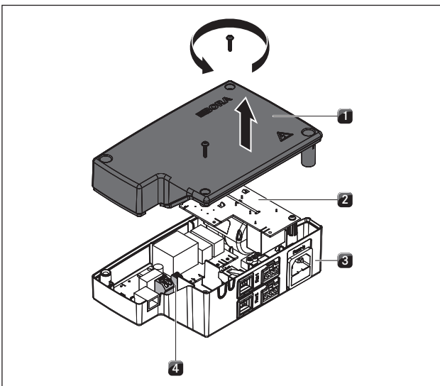
Fig. 6.38 Open the universal control unit's cover
