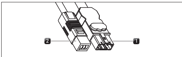
Fig. 6.48 Connection plug of the plinth fan
