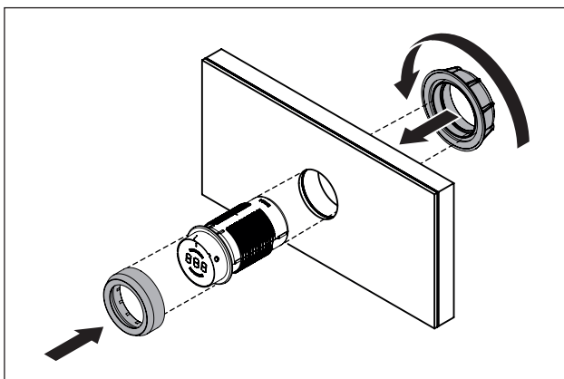
Fig. 6.23 Fitting the control knob
