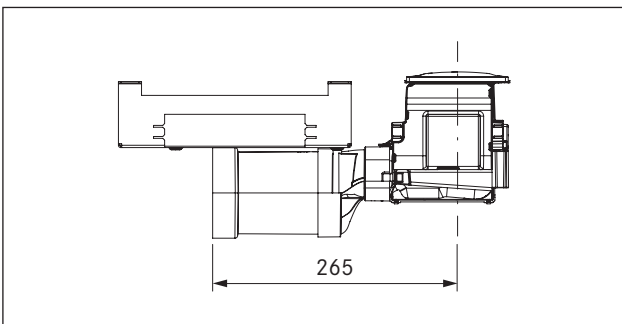
Fig. 6.17 PKA duct connection dimensions with straight ducting piece
