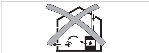
Fig. 6.35 Exhaust air installation – not permitted
