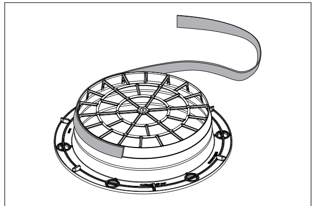
Fig. 6.31 Sealing tape position for installation with a round duct
