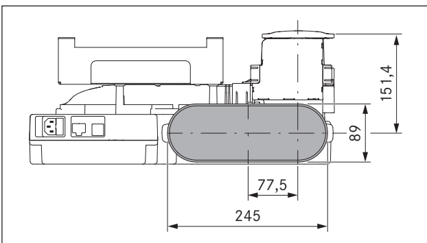
Fig. 6.18 PKAS, PKASAB duct connection dimensions
