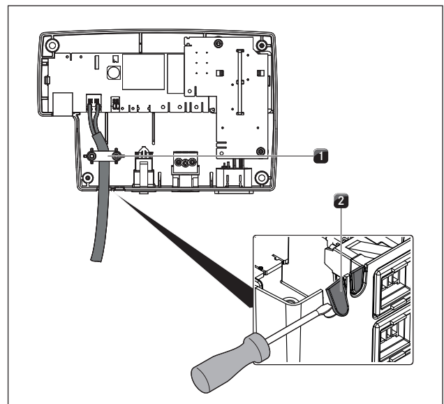
Fig. 6.42 Home Out contacts with strain relief
