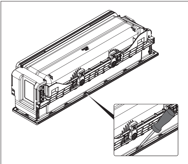
Fig. 6.29 Dismounting the cover frame
