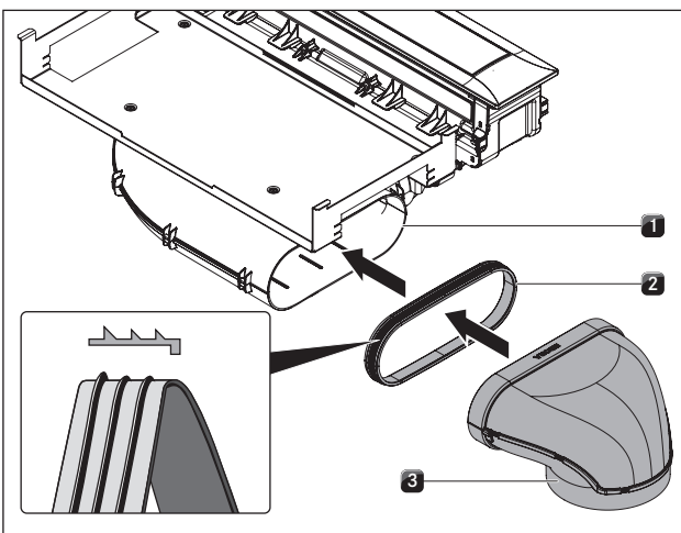
Fig. 6.33 Connecting to the duct system.
