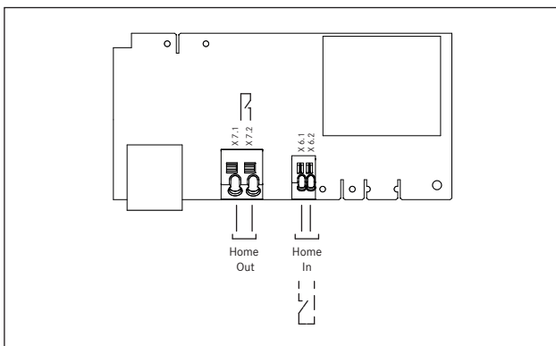
Fig. 6.41 Connection diagram for the external switch contacts
