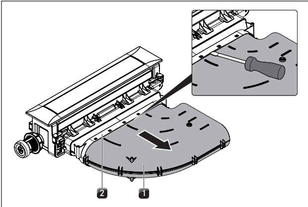
Fig. 6.25 Remove the angled ducting piece
