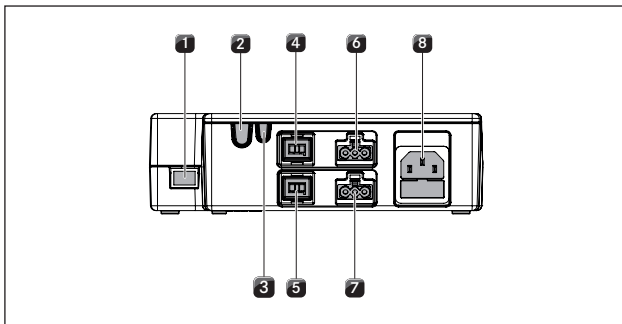
Fig. 6.47 Connections on the universal control unit
