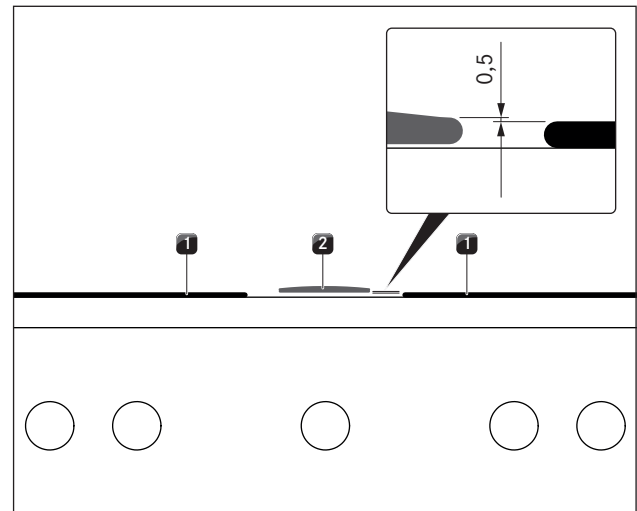
Fig. 6.10 Installing the cooktop extractor
