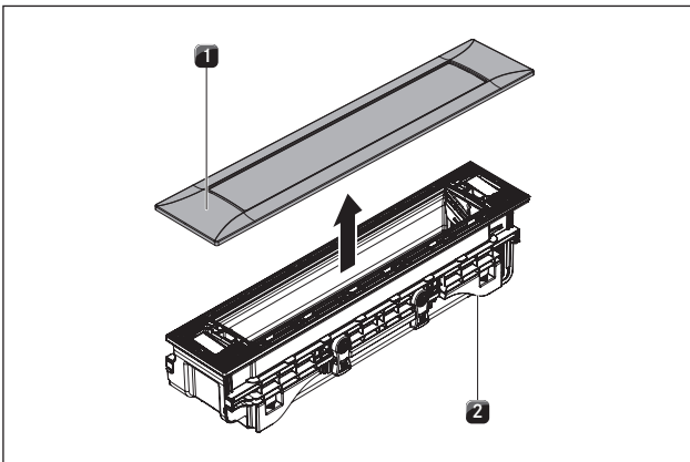
Fig. 6.30 Dismounting the cover frame
