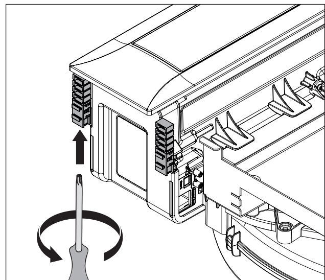
Fig. 6.14 Tighten the mounting clamps
