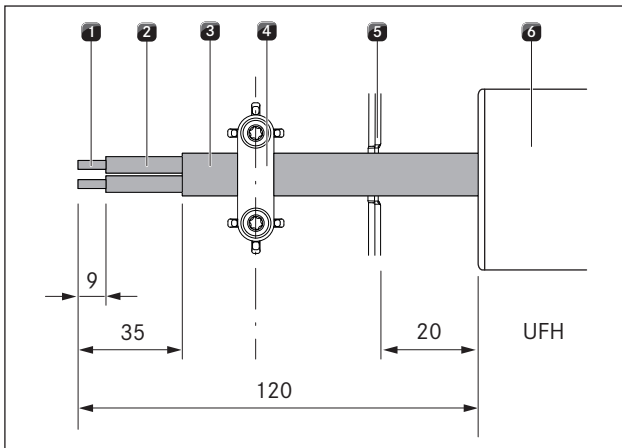
Fig. 6.40 Stripping lengths and installation position for connection cable
