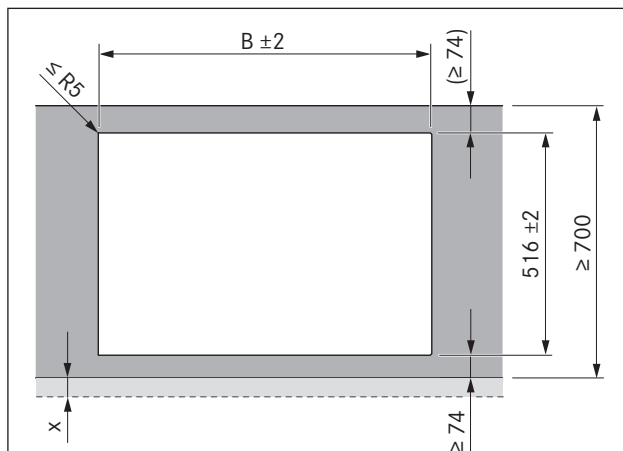
Fig. 6.5 Cut-out dimensions surface mounting
