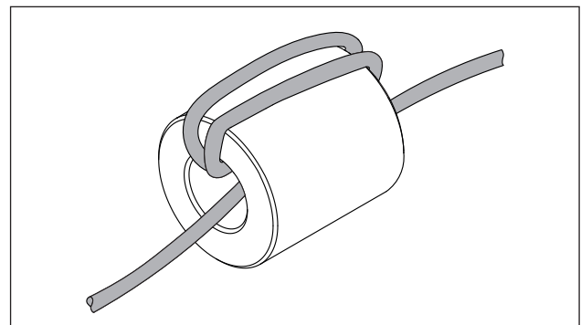
Fig. 6.39 Wrap the connection cable round the ferrite sleeve three times
