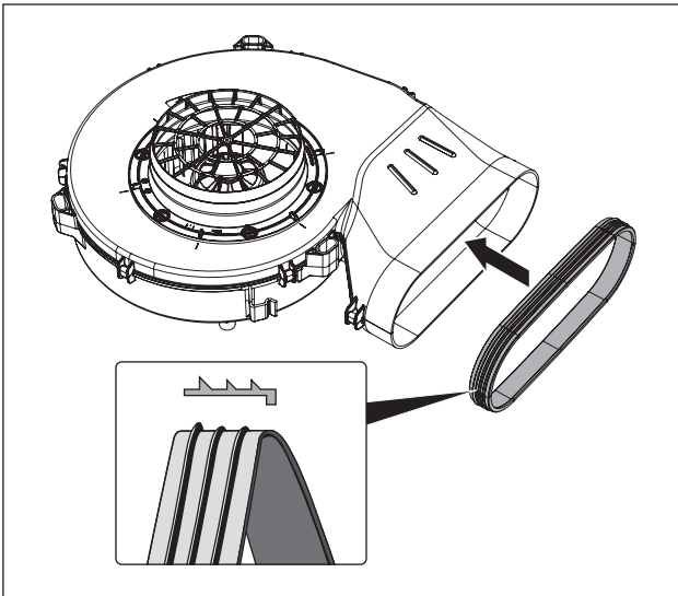
Fig. 6.32 Applying seal to the inlet nozzles of the plinth fan.
