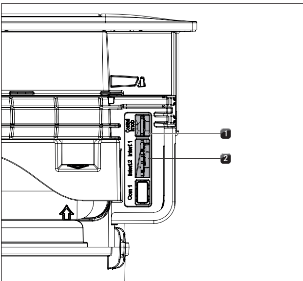
Fig. 6.44 Side connections on cooktop extractor
