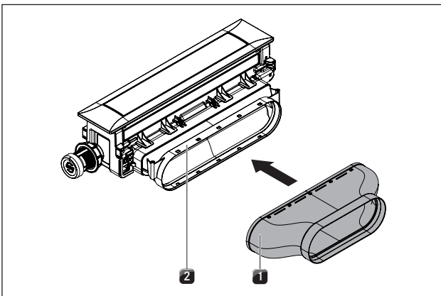
Fig. 6.26 Mounting the straight ducting piece
