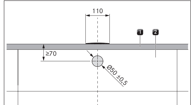
Fig. 6.19 Drill template
