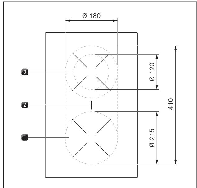
Fig. 4.15 Size of the cooking zones
