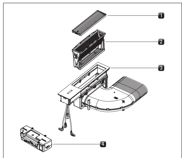
Fig. 4.5 BORA Classic cooktop extractor CKA2
