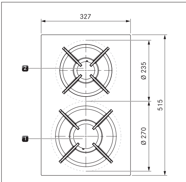
Fig. 4.17 Size of the cooking zones
