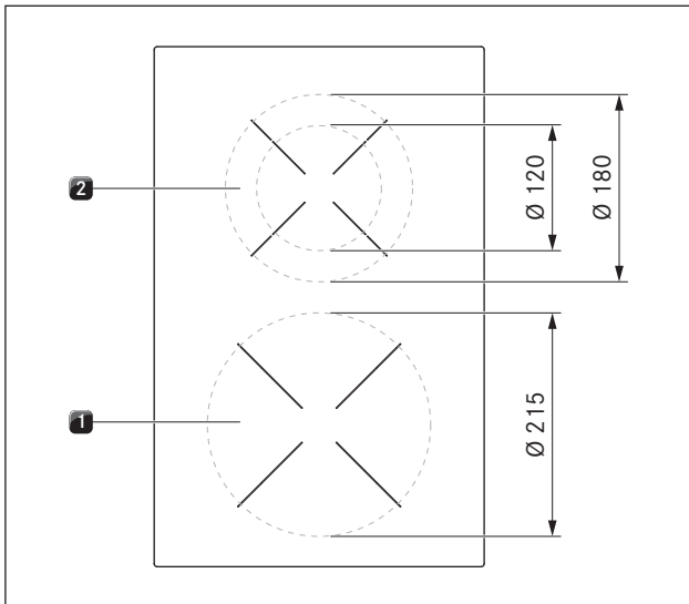
Fig. 4.13 Size of the cooking zones
