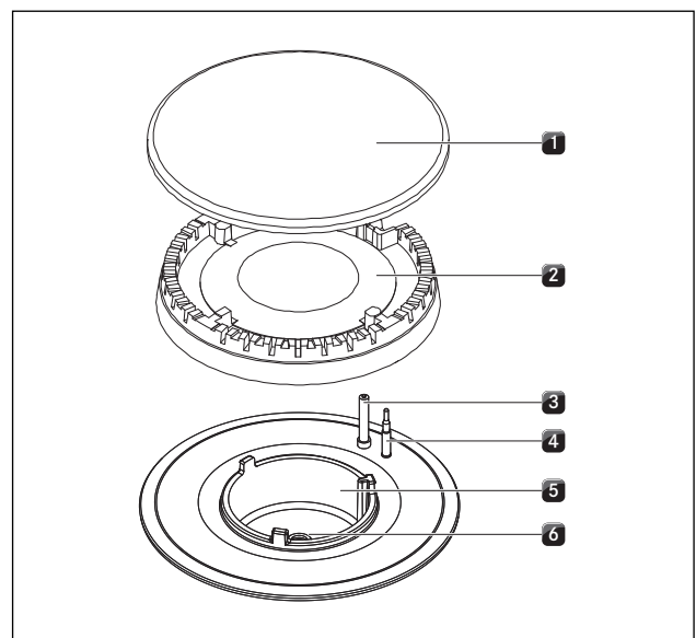
Fig. 9.2 Gas burner structure
