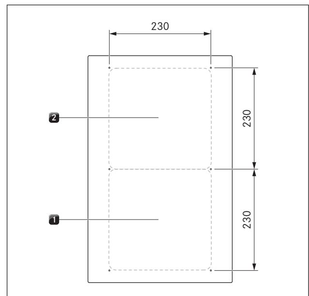
Fig. 4.7 Size of the cooking zones
