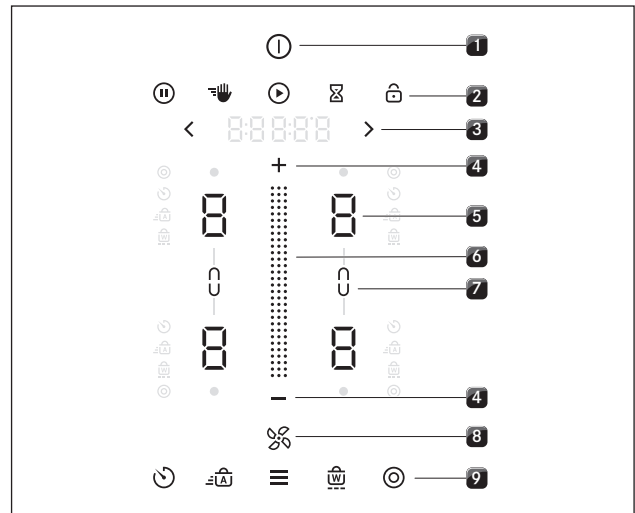
Fig. 4.2 Touch zones
