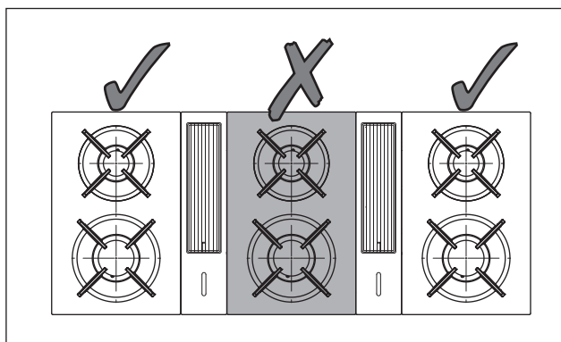
Fig. 4.5 Positioning the CKG with two cooktop extractors
