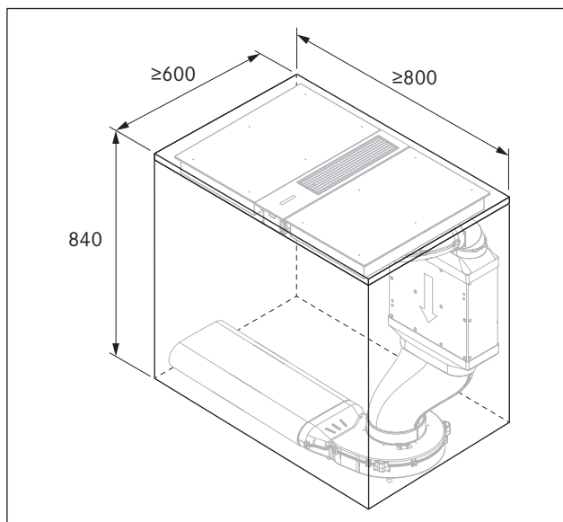
Fig. 4.14 Minimum installation dimensions with shallow silencer USDF
