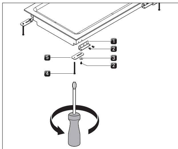
Fig. 4.32 Securing the Tepan stainless steel grill
