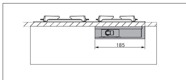
Fig. 4.8 Side cut-out for the gas connection
