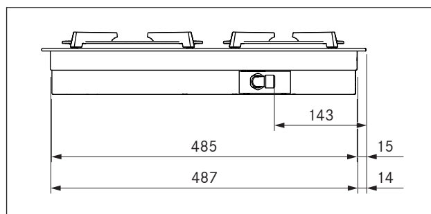
Fig. 3.22 CKG device dimensions side view
