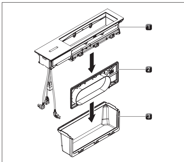
Fig. 4.22 Assembling the individual components on cooktop extractor CKA2/CKA2AB
