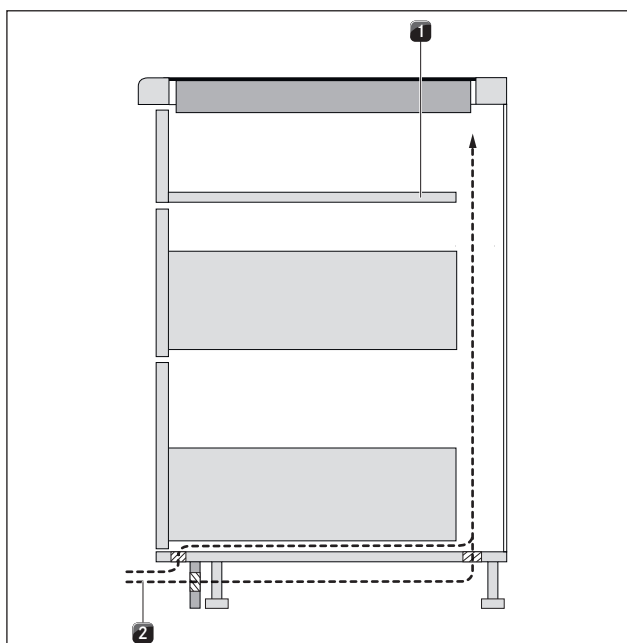
Fig. 4.7 Plinth area air supply
