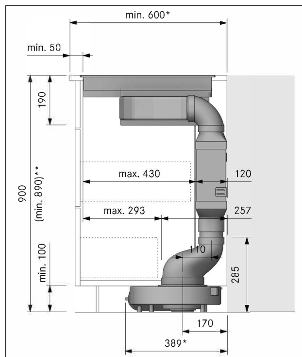
Fig. 4.14 Minimum installation dimensions with shallow silencer USDF
