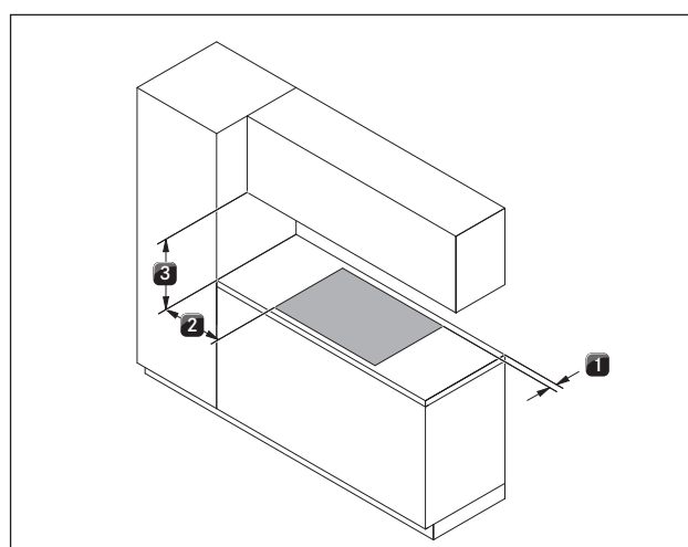
Fig. 4.3 Minimum distance
