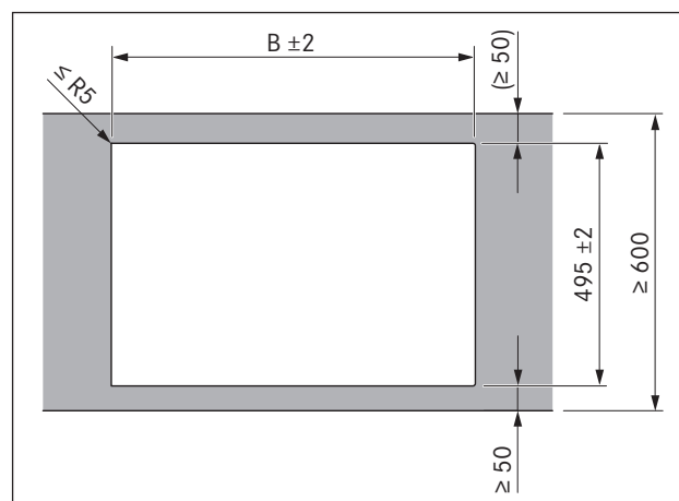
Fig. 4.12 Cut-out dimensions for surface mounting
