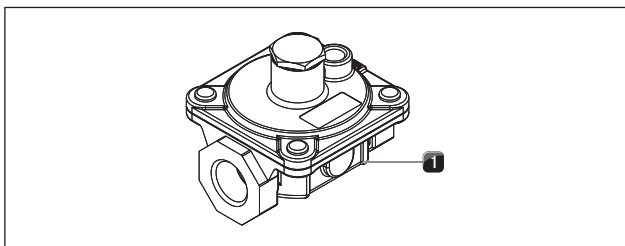
Fig. 4.46 Connection with gas regulator (NG)
