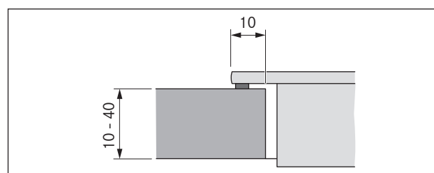
Fig. 4.13 Dimension of support for surface mounting
