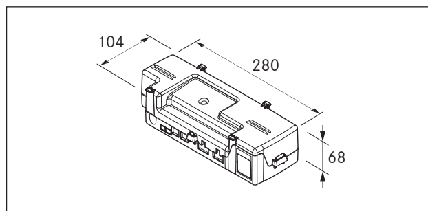
Fig. 3.4 Device dimensions control unit
