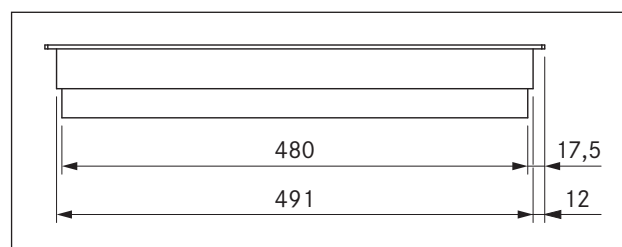
Fig. 3.19 CKCB device dimensions side view
