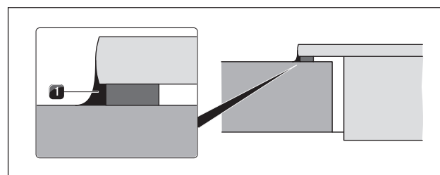
Fig. 4.52 Silicone sealant for surface mounting
