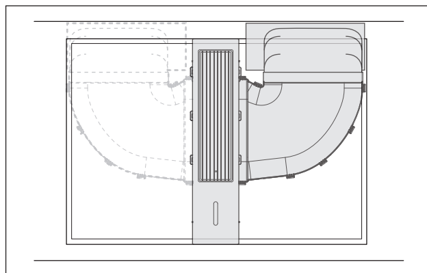
Fig. 4.19 Airflow towards the rear (right or left)
