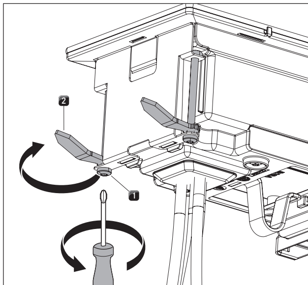
Fig. 4.30 Securing the cooktop extractor
