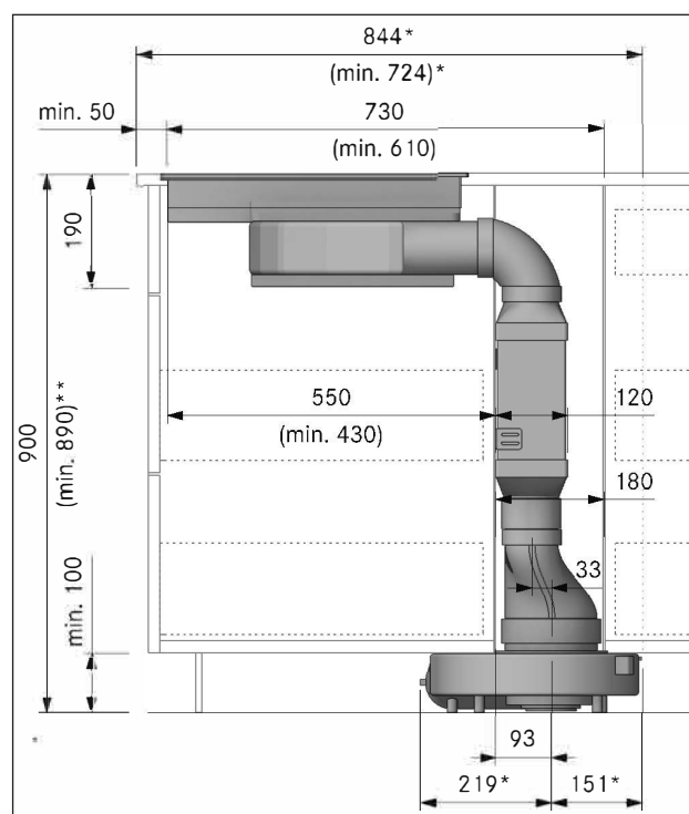
Fig. 4.16 Appliance installation dimensions with shallow silencer USDF, duct connection flat EFV and transition, flat round offset EFRV110 (kitchen counter 600)
