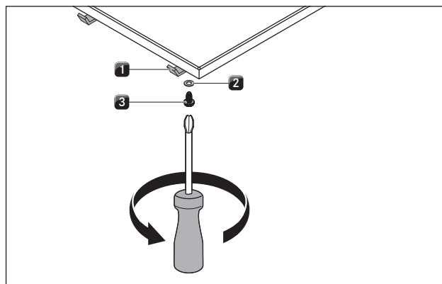
Fig. 4.31 Securing the cooktops
