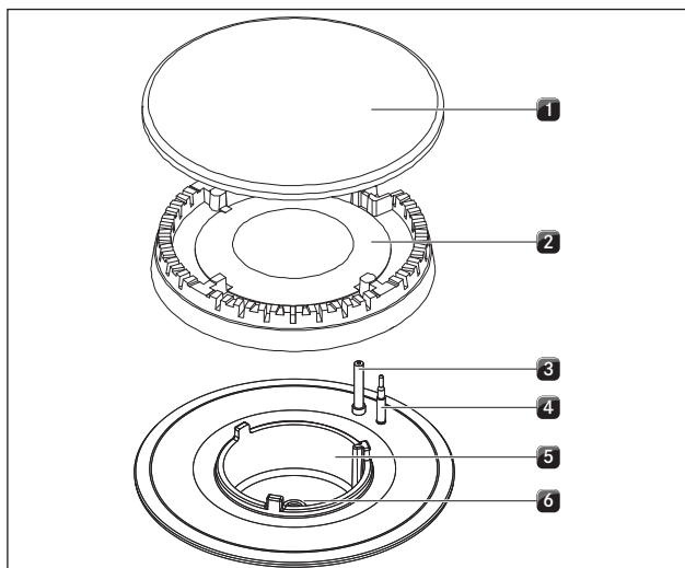
Fig. 4.48 Gas burner structure
