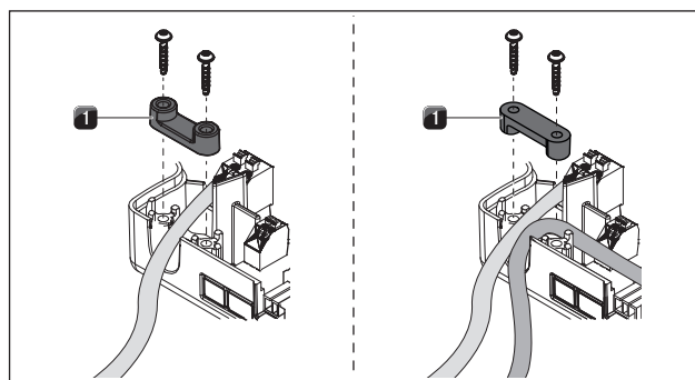
Fig. 4.37 Fitting the strain relief clamp
