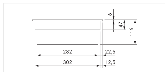
Fig. 3.12 CKIW device dimensions front view
