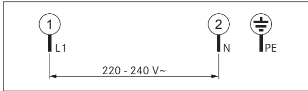
Fig. 4.44 Connection diagram 1-phase connection cooktop
