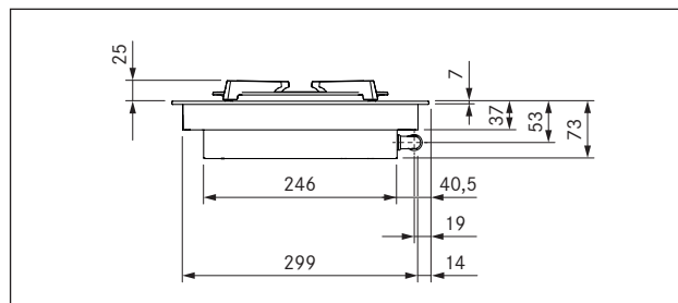
Fig. 3.21 CKG device dimensions front view
