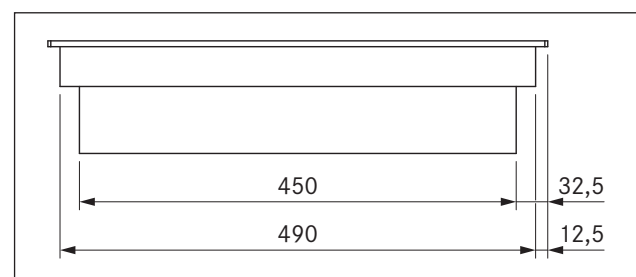
Fig. 3.13 CKIW device dimensions side view
