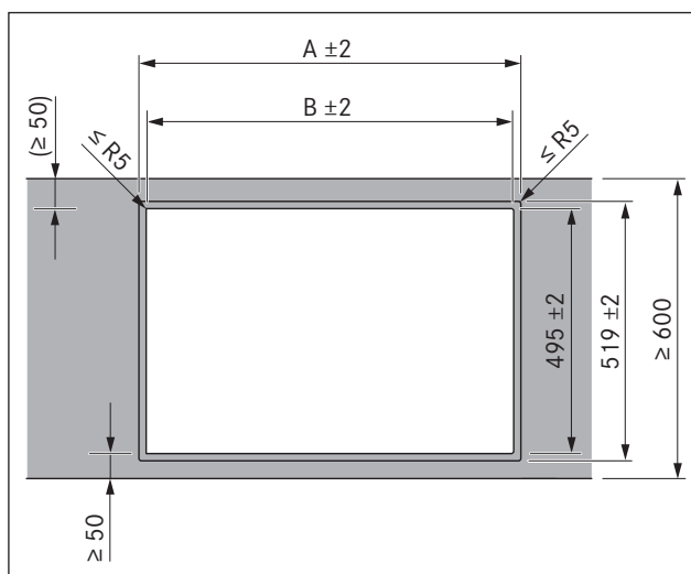
Fig. 4.10 Cut-out dimensions for flush installation
