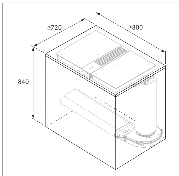
Fig. 4.15 Minimum installation dimensions with round silencer USDR50
