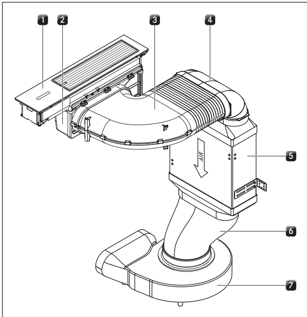
Fig. 4.27 Cooktop extractor CKA2/CKA2AB standard set-up
