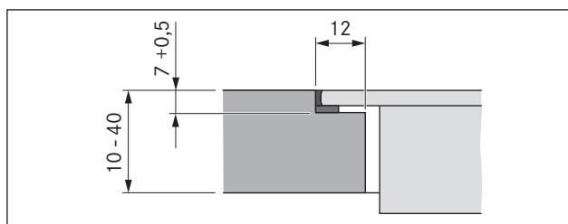
Fig. 4.11 Groove dimensions for flush installation
