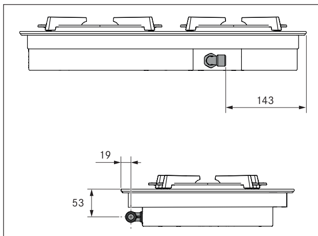
Fig. 4.45 Position of gas connection
