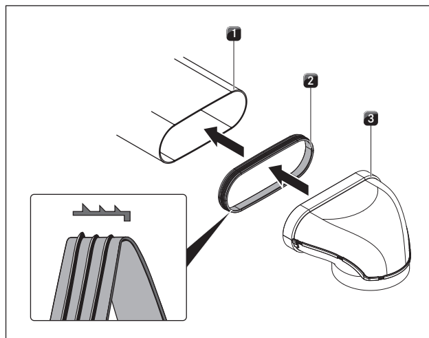
Fig. 4.26 Assembly of the duct system
