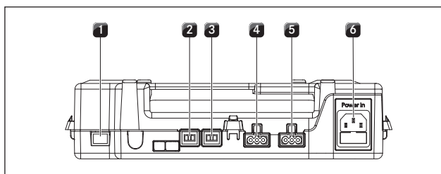
Fig. 4.42 Control unit connections
