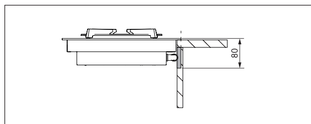
Fig. 4.9 Side cut-out for the gas connection (front view)
