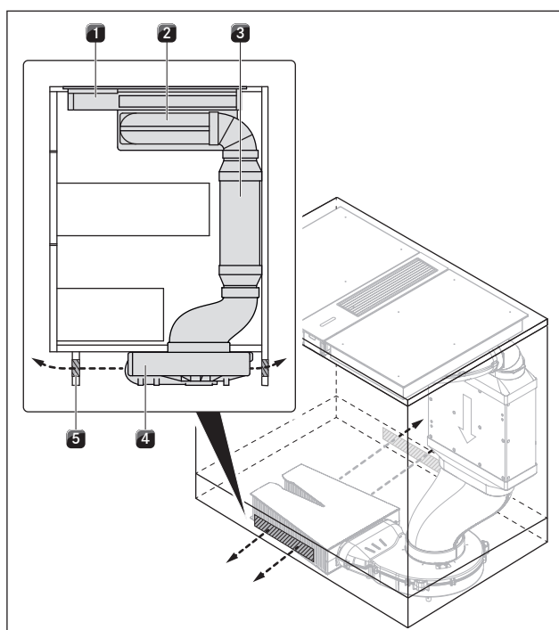
Fig. 4.4 Recirculation design example (kitchen island + cooktop + CKA2/ /CKA2AB + air cleaning unit)
