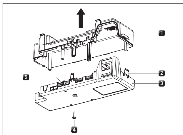
Fig. 4.33 Opening the control unit housing cover
