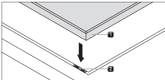
Fig. 4.29 Cooktop and height adjustment plates
