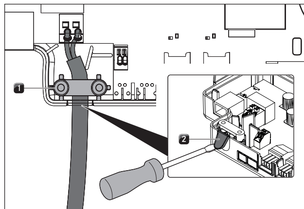
Fig. 4.36 Home Out contacts with strain relief
