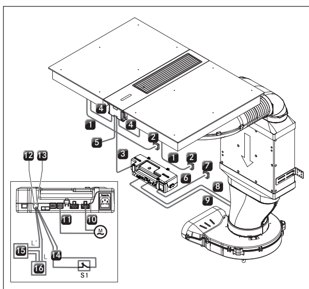
Fig. 4.38 Connection diagram for cooktop extractor CKA2/CKA2AB
