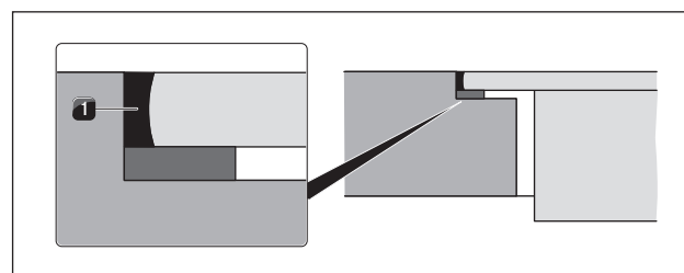
Fig. 4.51 Silicone sealant for flush installation
