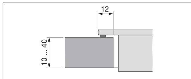
Fig. 5.6 Surface mounting cut
