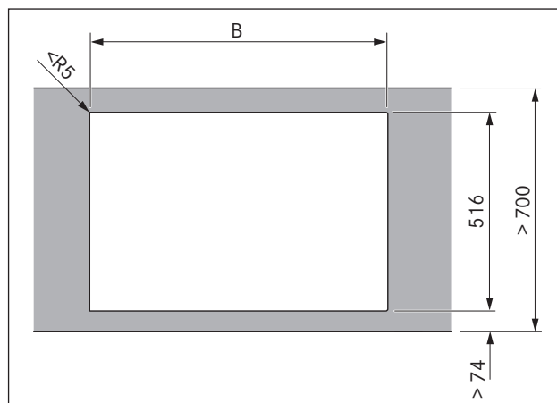
Fig. 5.5 Surface installation
