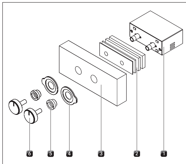
Fig. 5.9 Control box structure
