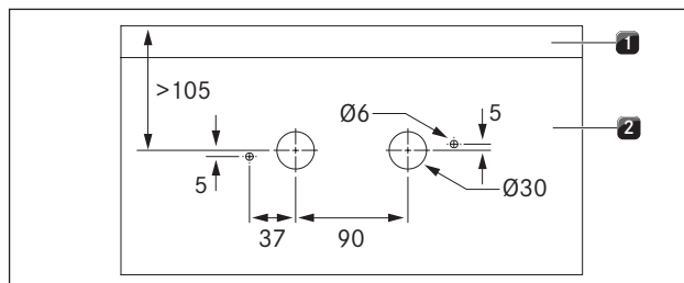
Fig. 5.10 Drilling template
