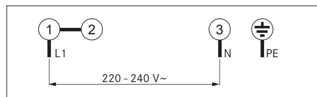
Fig. 5.18 Connection diagram 1-phase
