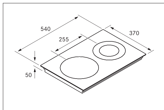
Fig. 3.1 Device dimensions
