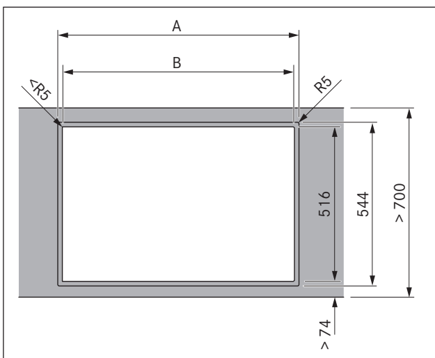
Fig. 5.3 Planlimet montering
