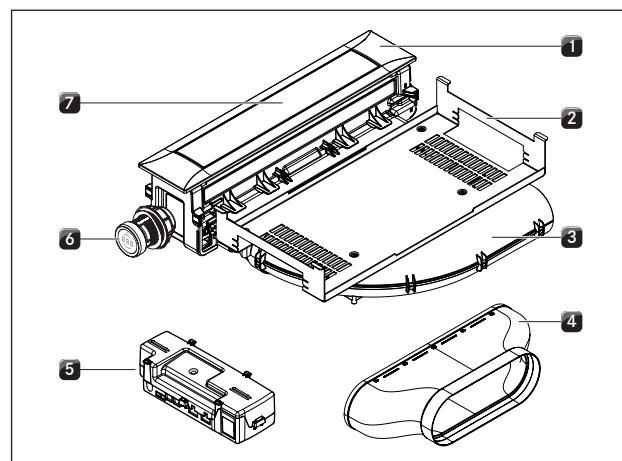
Afb. 4.5 Kookveldafzuiging PKA3/PKA3AB
