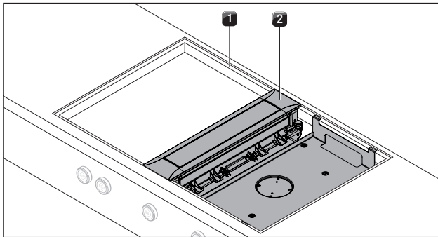
Afb. 4.25 Kookveldafzuiging inleggen
