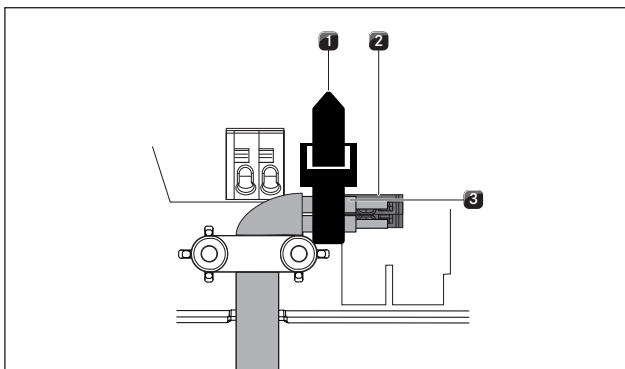
Afb. 4.46 Kabelbinder Home In-interface PKAS3/PKAS3AB
