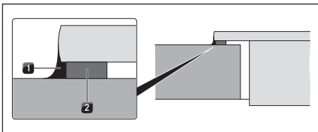
Fig. 10.30 Sealing tape in the case of surface mounting
