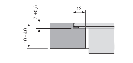
Fig. 10.7 Rebate dimensions for flush installation
