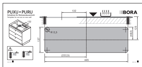
Fig. 10.28 Template for back panel cut-out
