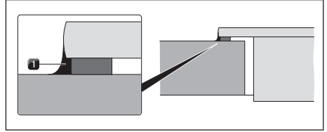
Fig. 10.54 Silicone sealant for surface mounting
