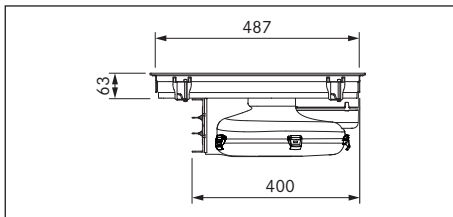
Fig. 3.9 PURA device dimensions side view
