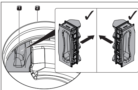
Fig. 10.44 Inserting the filter replacement cover
