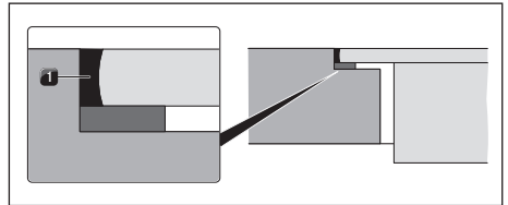
Fig. 10.55 Silicone sealant for flush installation
