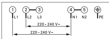
Fig. 10.47 Connection diagram - two-phase connection
